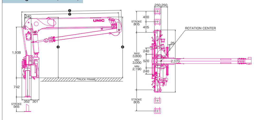
Drawing: UR-V504 (Unit: mm)
